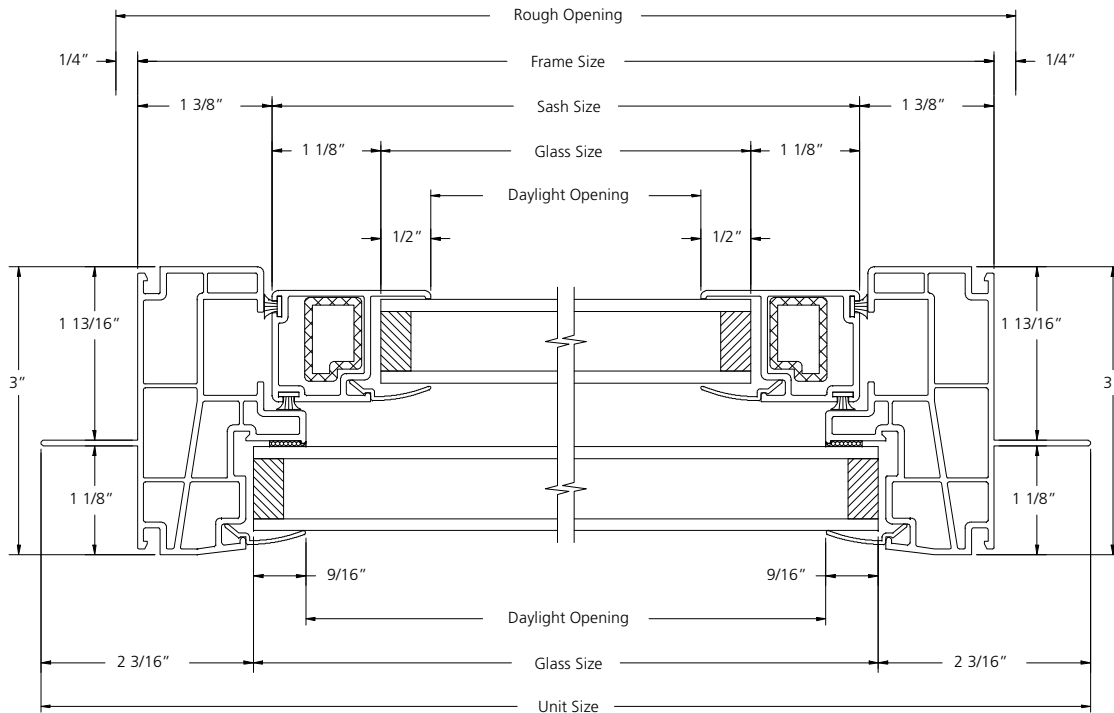
HORIZONTAL SECTION
