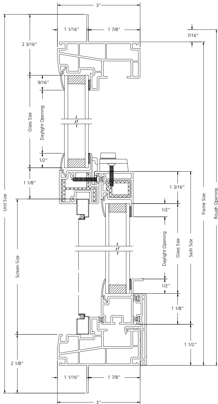
VERTICAL SECTION
