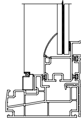
MONO GLAZED IMPACT GLASS 7/16" GLASS SIZE
