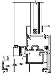
3/4" LAMINATED GLASS 3/16" GLASS SIZE
