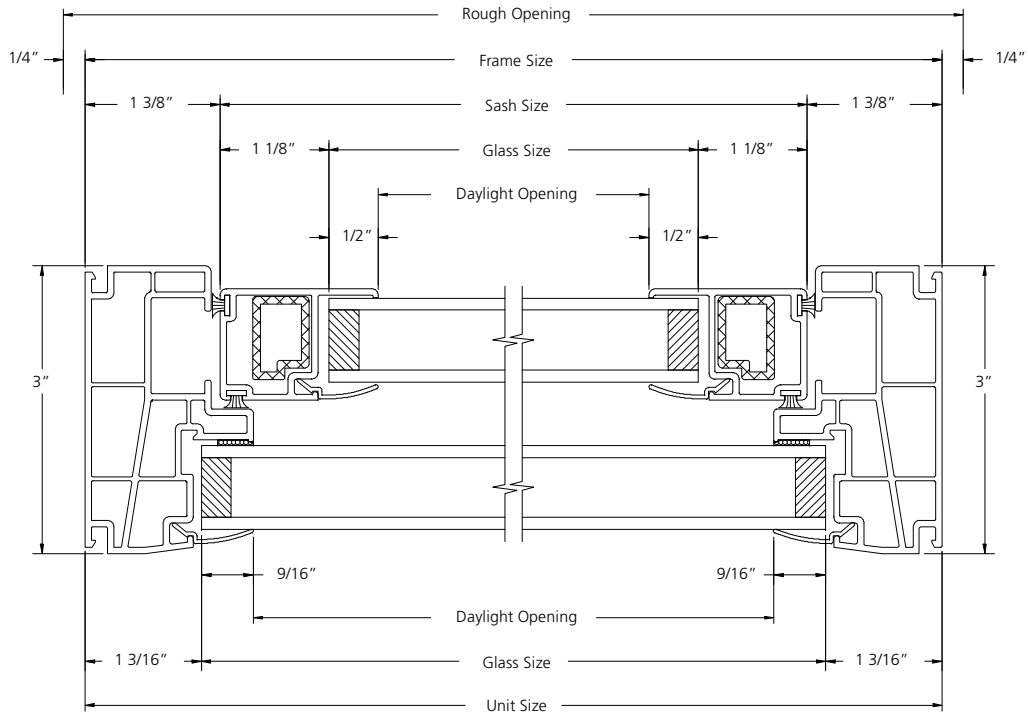
HORIZONTAL SECTION
