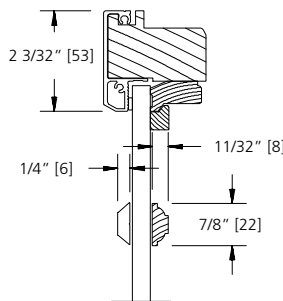
7/8" SDL (PUTTY LINE)
