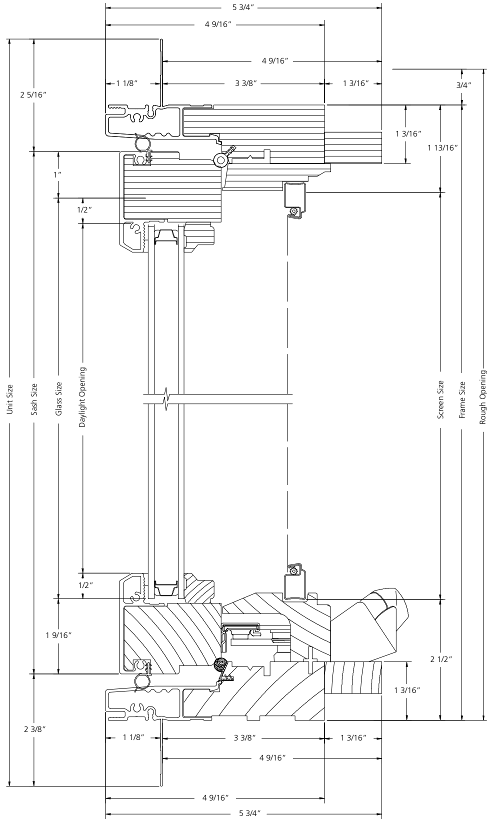
VERTICAL SECTION
