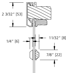
7/8" SDL (PUTTY LINE)
