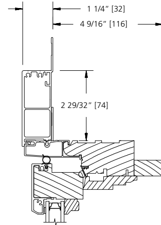
3 1/2" FLAT CASING
