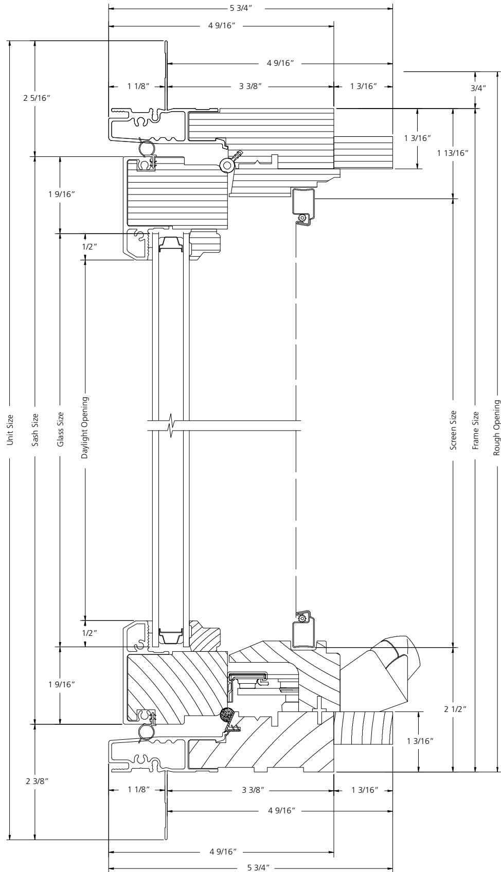
VERTICAL SECTION
