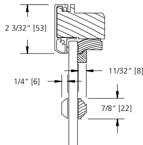
7/8" SDL (PUTTY LINE)
