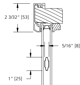
1" CONTOUR GBG
