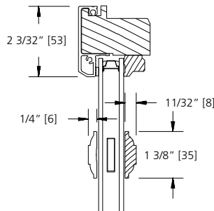
1 3/8" SDL BAR (BEAD STOP)
