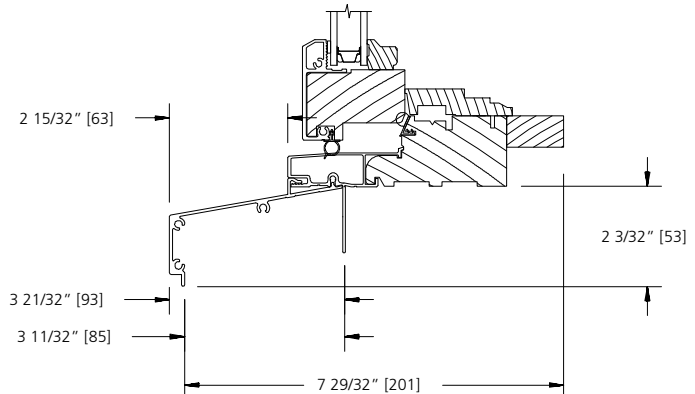
EXTENDED SILL NOSE
