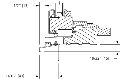
SILL NOSE
