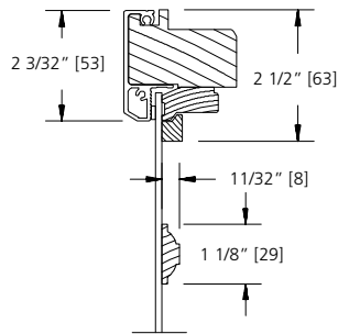
1 1/8" GRILLE BAR
