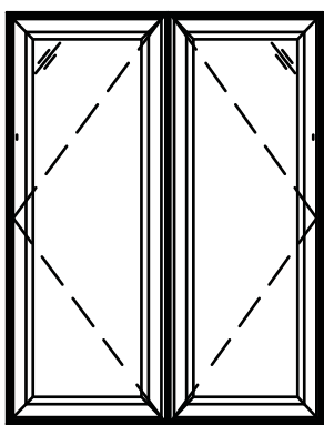
Twin Casement Units 73 1/4 x 64" v-600
