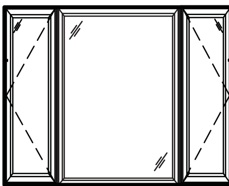
Triple XOX Casement 96" x 64" v-600 & v-630 Factory Units with Integral Frame Mullions
